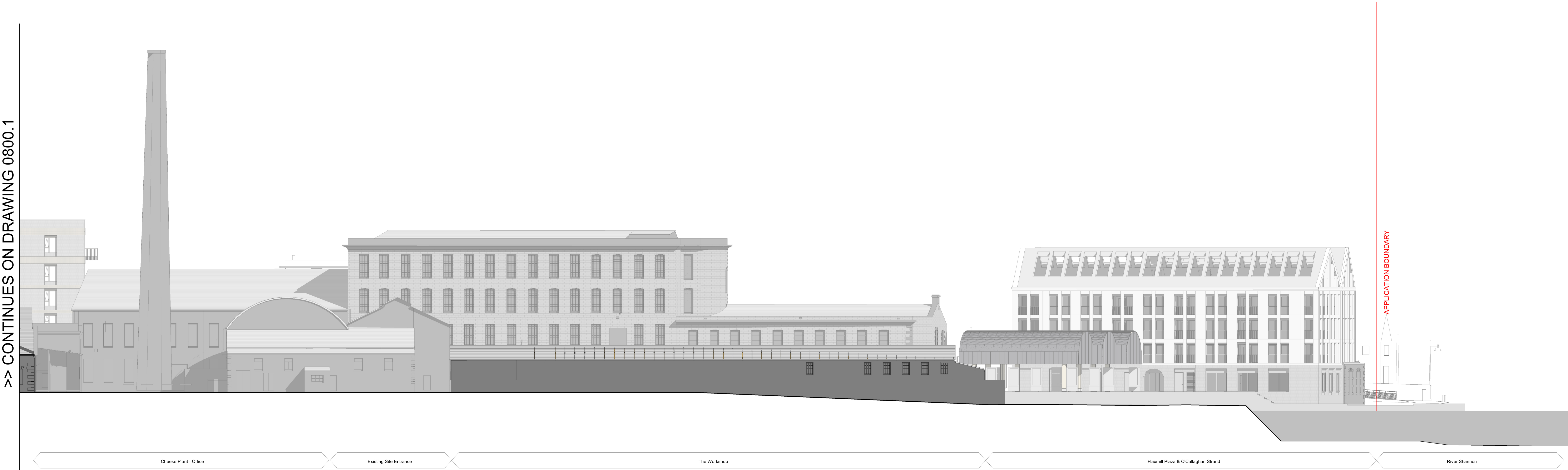
2 Proposed Site Elevation 01 - B2 1 : 200
